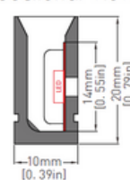
Sectional View
