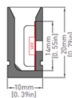
Sectional View
